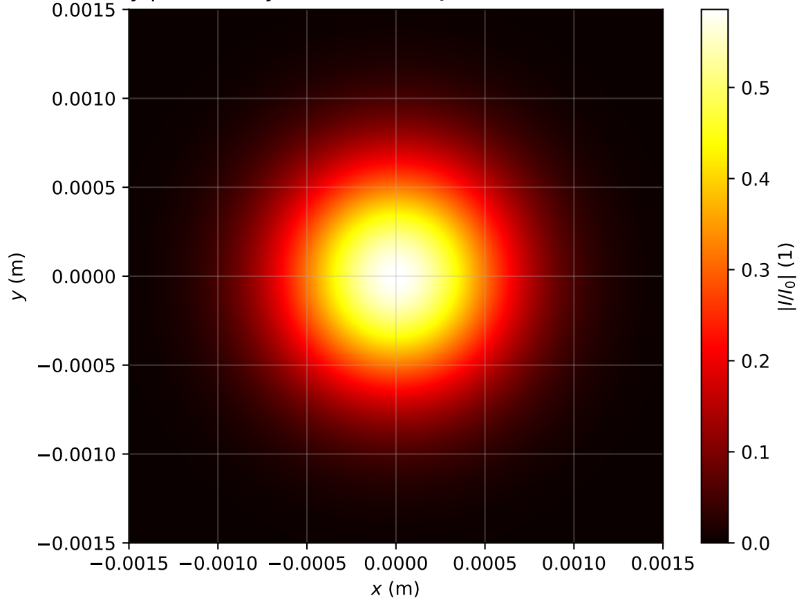
Intensity profile I(x, y, z = 1.831m)/I_0 , \text{Pin}=0.1\text{Pcr} , artificial time
